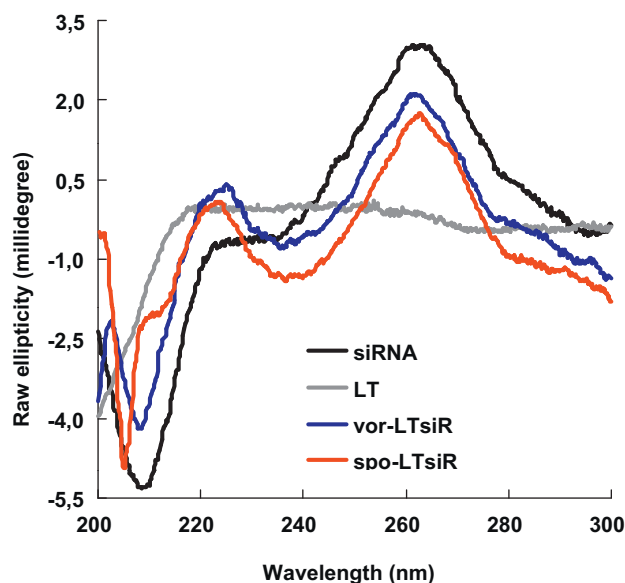
Fig. 2. Effect of preparation procedure on the CD spectra of siRNA in the lipoplex. Cationic lipid + /siRNA − ratio was 9.6 \mu M/30 nM, which corresponds to a charge ratio of 7.62. The data are typical of 3 independent experiments.
