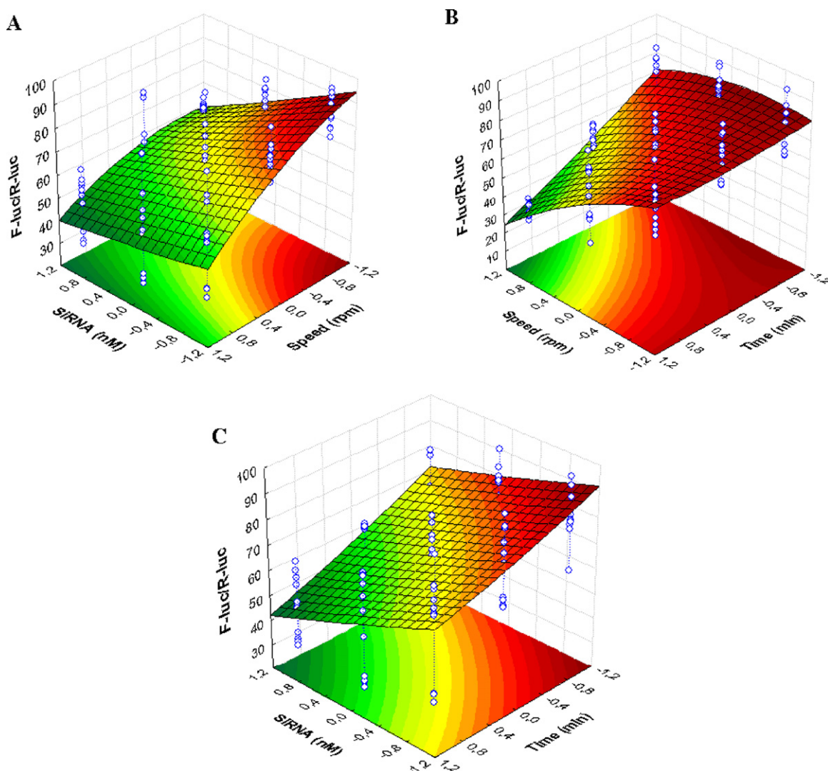
Fig. 3. Response surface plots showing the effect of siRNA dose and vortex speed (A), the effect of vortex speed and vortex time (B), and the effect of siRNA dose and vortex time (C) on the in vitro luciferase gene knockdown effect.
